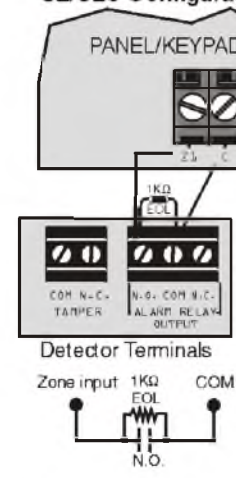
N.O., With EOL UL/ULC Configuration
