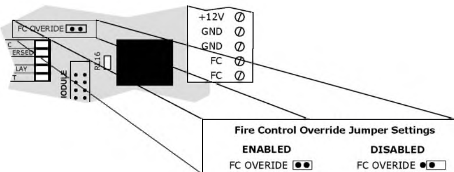
Figure 11: Fire Control (FC) Override Jumper:
