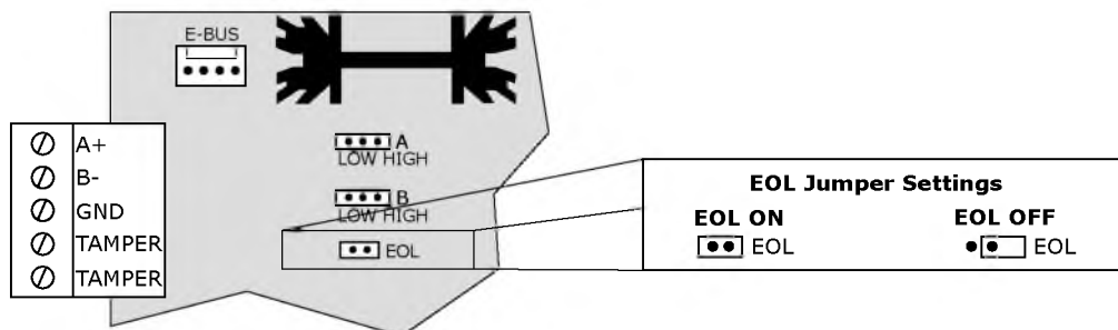
Figure 9: EOL Jumper Settings:
