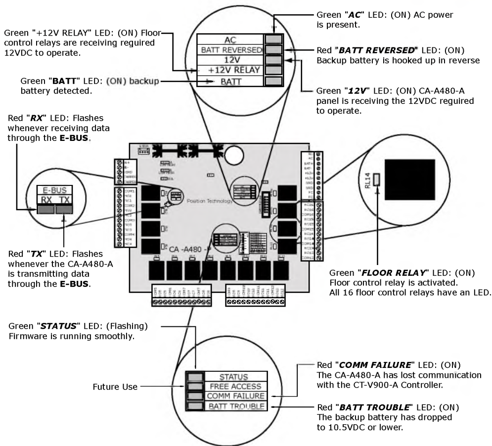
Figure 18: CAA480A's LEDs:
