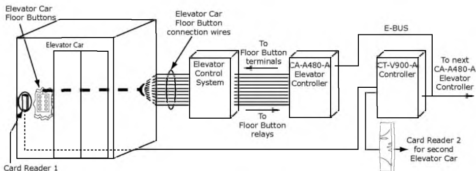
Figure 5: Standard Button Control (Fail Safe):
